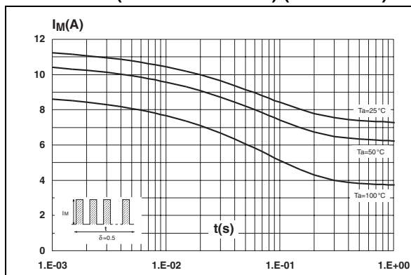
Figure 7. Non repetitive surge peak forward current versus overload duration (maximum values) (DO-201AD)
