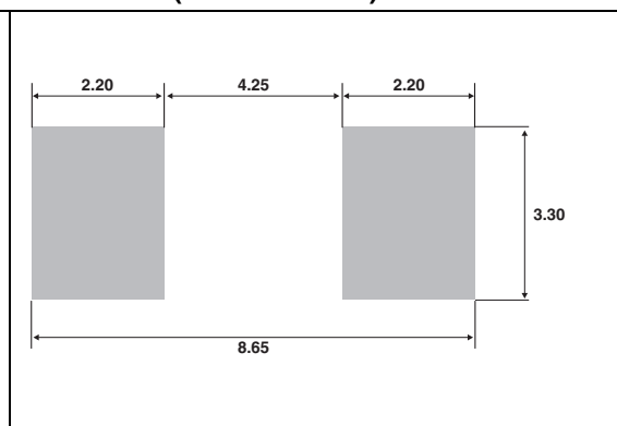
Figure 20. SMC footprint dimensions (in millimetres)
